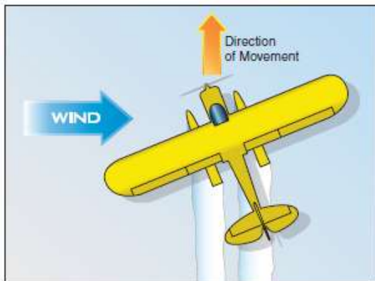
Figure 7-5. Crosswind taxi.
