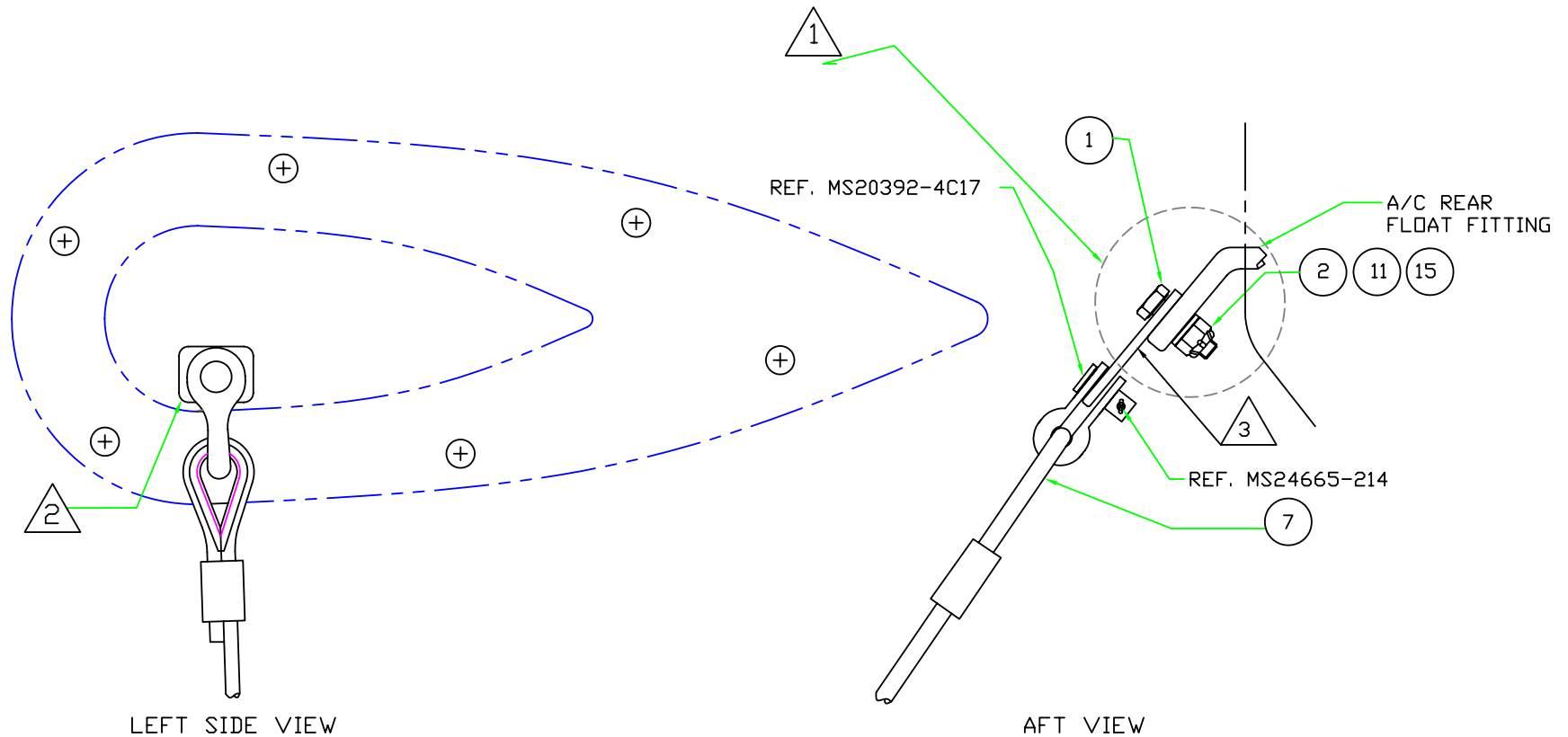
DETAIL B: REAR CHECK CABLE ATTACHMENT, TOP
