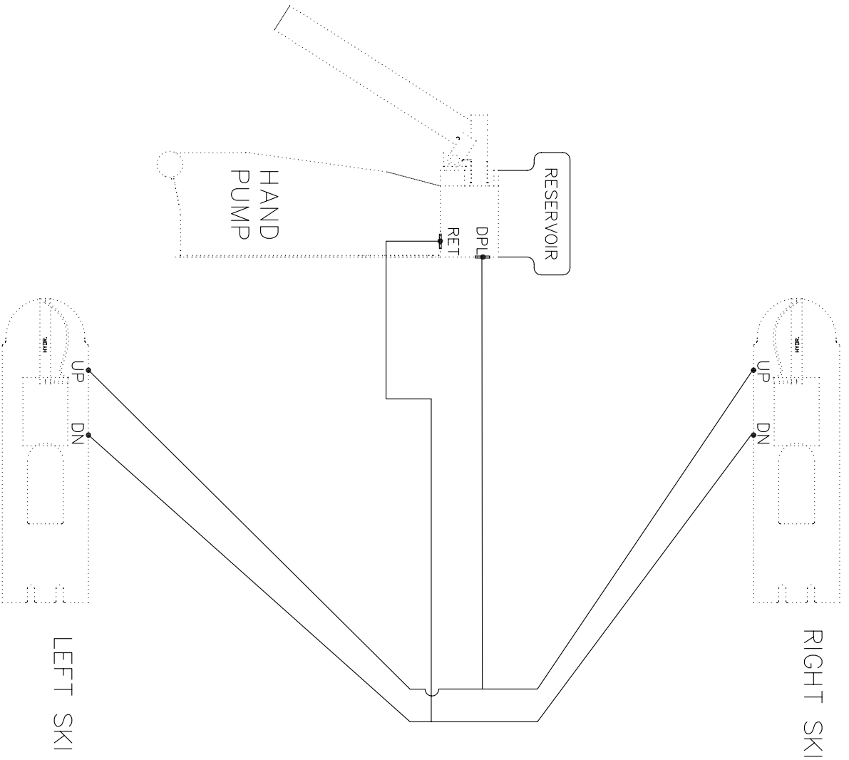
1010-02: HYDRAULIC SCHEMATIC FOR HAND PUMP ONLY OPTION
