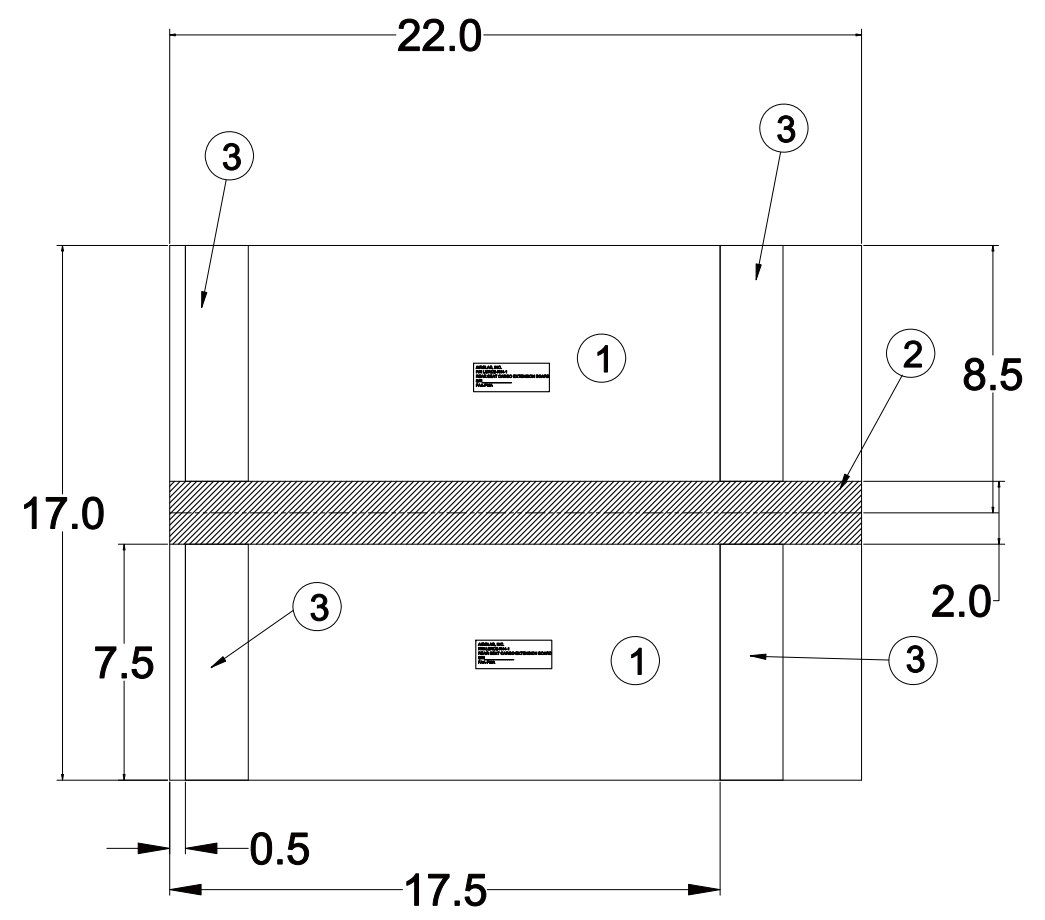
LRSCE-R44 REAR SEAT CARGO EXTENSION (BOTTOM SIDE DEPICTED)
