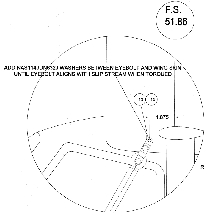
DETAIL D LEFT SHOWN RIGHT OPPOSITE
