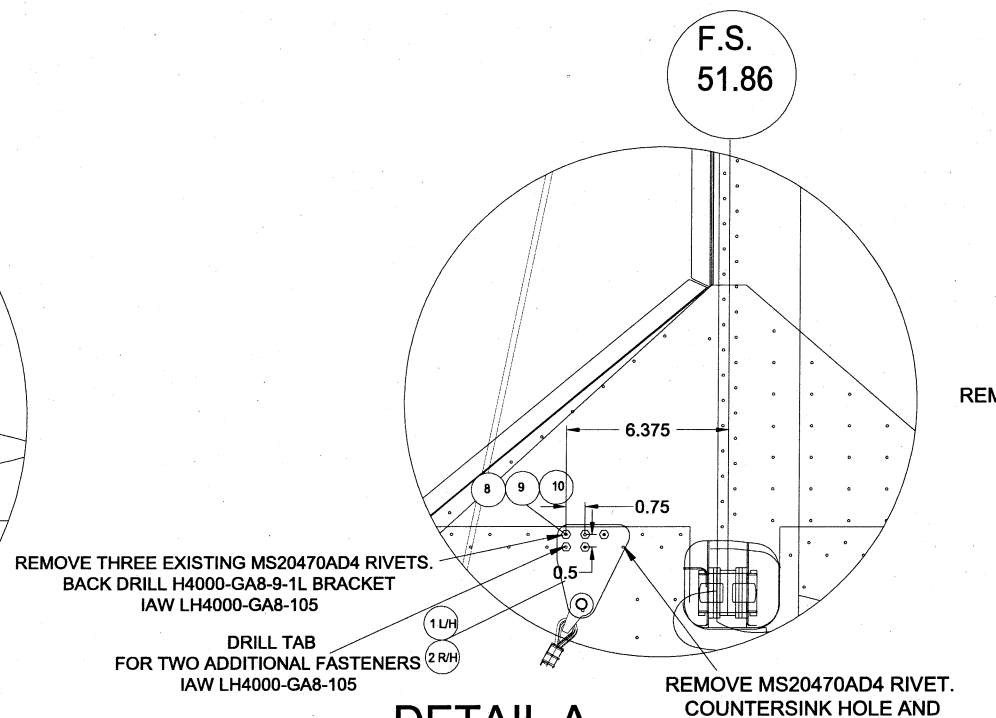
DETAIL A LEFT SHOWN RIGHT OPPOSITE
