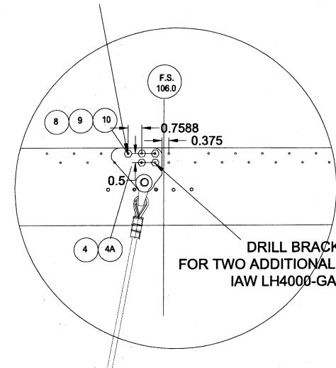
DETAIL C RIGHT CHECK CABLE
