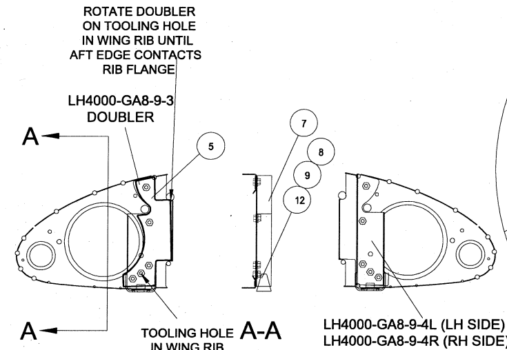
BUNGEE ATTACH BRACKET IN WING LH SHOWN-RH OPPOSITE
