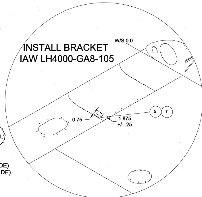
DETAIL E RIGHT SHOWN LEFT OPPOSITE
